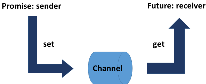
Tasks as data channels between communication endpoints
