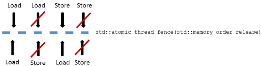
Release fence
