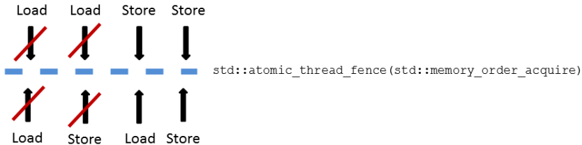
Fence with acquire semantic
