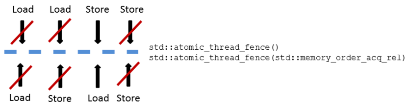
Full fence
