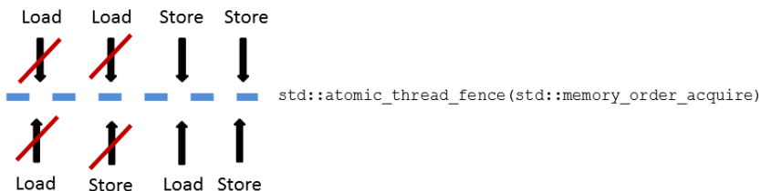
Acquire fence
