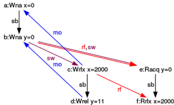
Execution for ( y = 0, x = 2000 )
