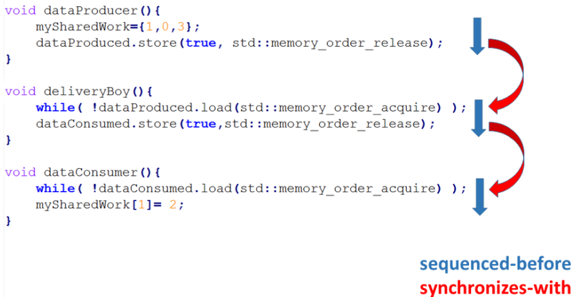
Transitivity of the acquire-release semantics
