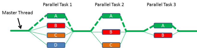
The fork-join paradigm
